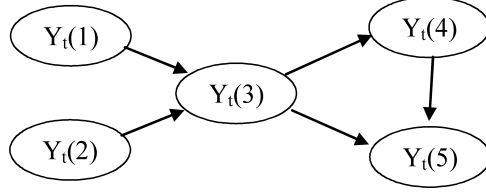
Figure 1: DAG representing five time series at time t .
