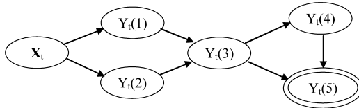
Figure 10: DAG representing time series of vehicle counts in Example 4, with an extra node \mathbf{X}_t to account for any correlation between Y_t(1) and Y_t(2) .
