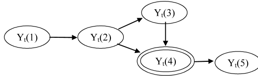
Figure 5: DAG with a logical node Y_t(4) .
