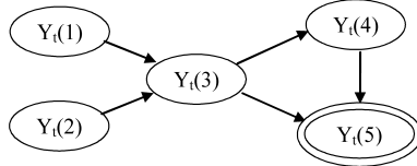
Figure 7: DAG representing the conditional independence relationships between Y_t(1), \dots, Y_t(5) in the traffic network of Figure 6.
