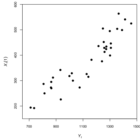
Figure 3: Plot of X_t(1) against Y_t .
