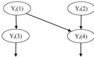
Figure 8: Part of a DAG for Example 3 for four time series Y_t(1), \dots, Y_t(4) .
