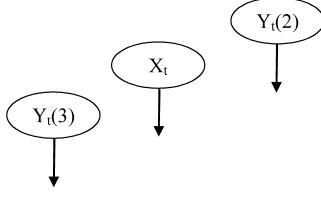
Figure 9: New DAG for Example 3 (adapting the DAG in Figure 8) where X_t is introduced into the DAG and Y_t(1) and Y_t(4) are no longer observed.
